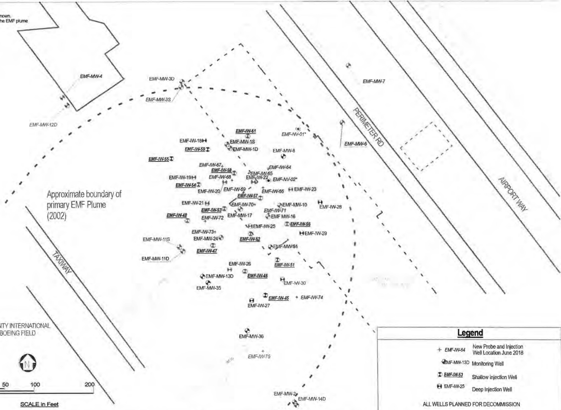
Figure 3 - EMF Monitoring and Injection Wells planned for Decommissioning
